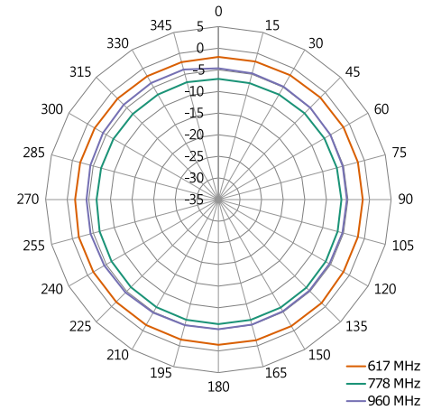
XY-Plane Gain
