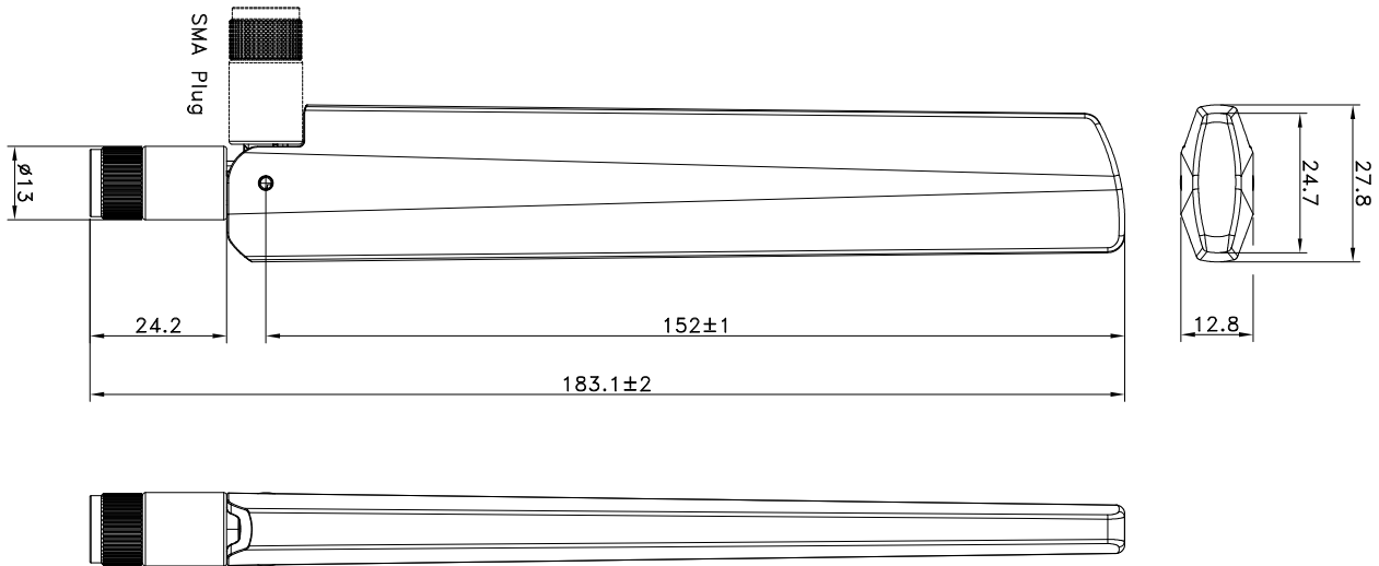
Figure 2. Antenna Dimensions
