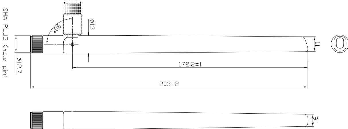
Figure 2. Antenna Dimensions
