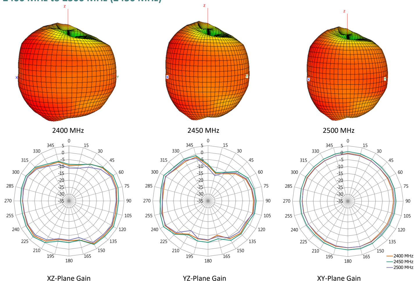
Figure 17. Antenna Radiation Patterns, Edge Bent 90 Degrees
