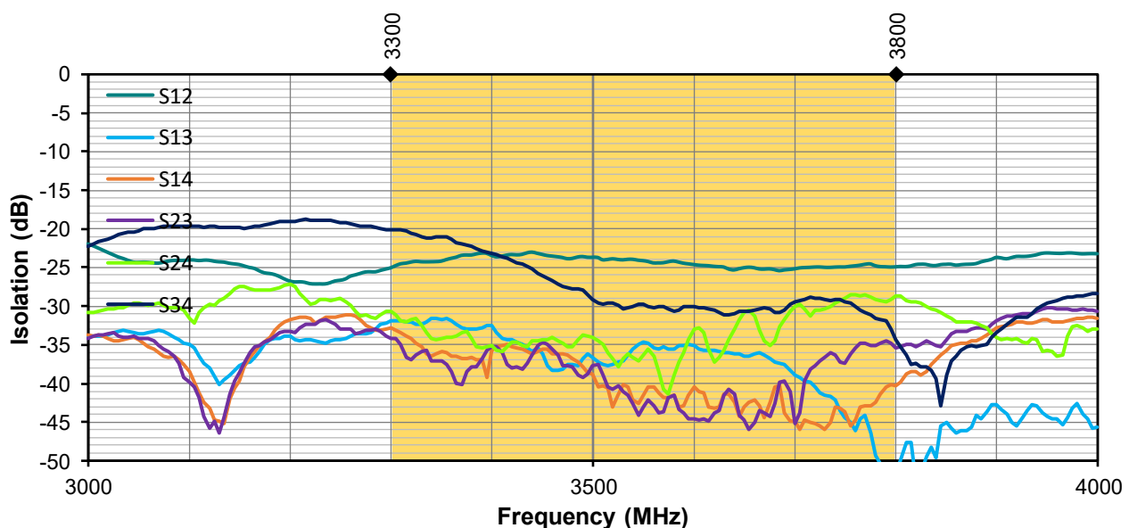
Figure 9. Antenna Isolation
