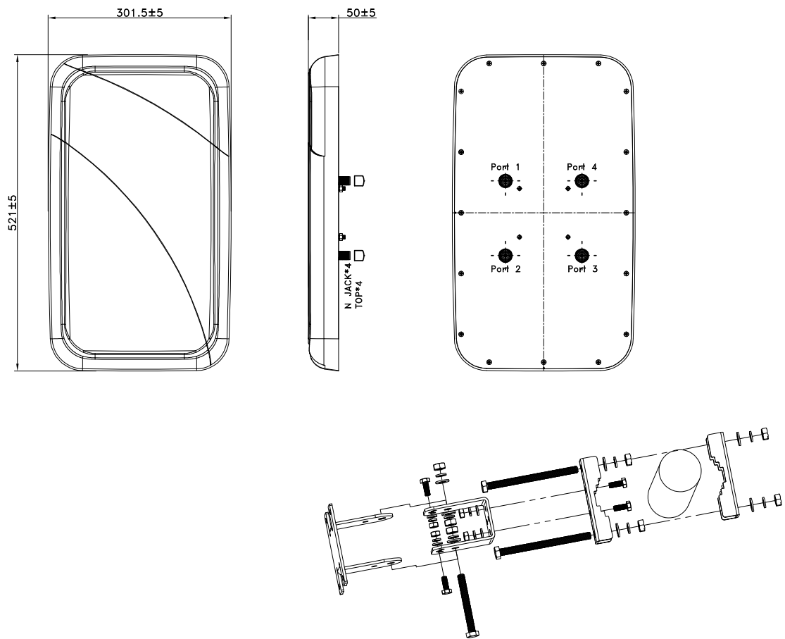
Figure 2. Antenna Dimensions
