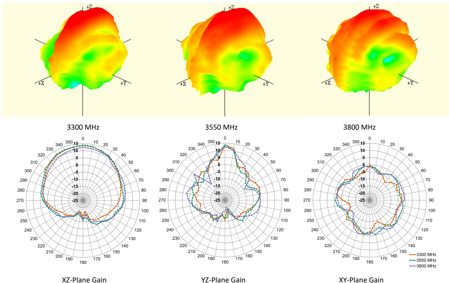
Figure 10. Antenna Radiation Patterns
