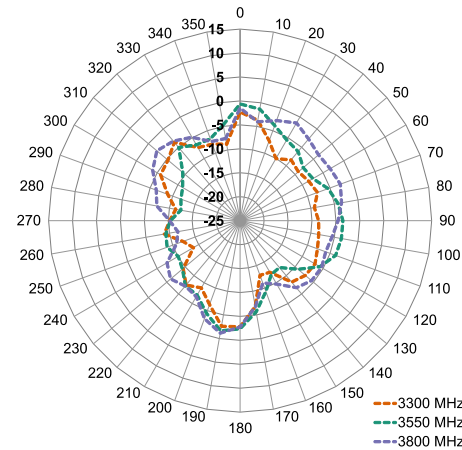
XY-Plane Gain
