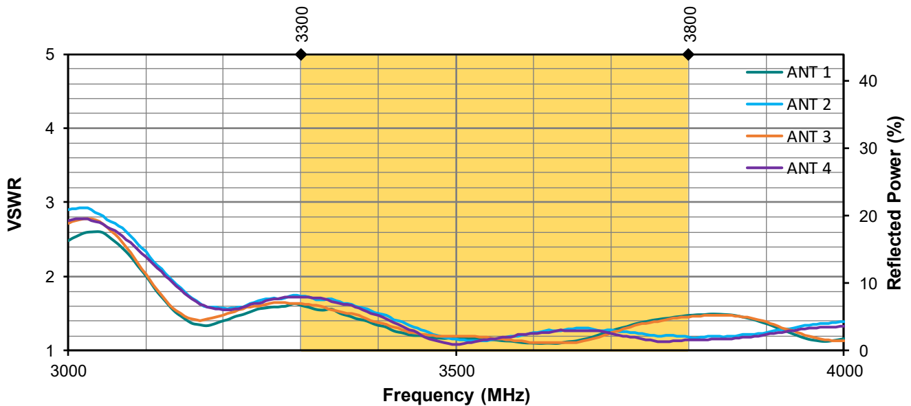
Figure 4. Antenna VSWR
