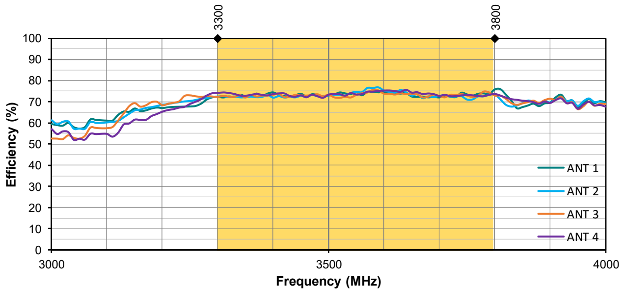
Figure 8. Antenna Efficiency
