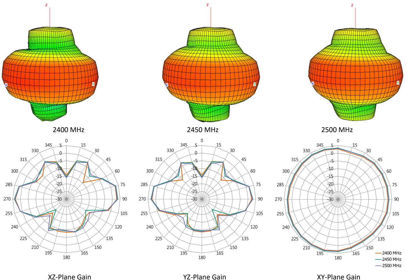
Figure 10. Antenna Radiation Patterns, Straight without ground plane
