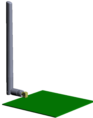
Figure 11. On edge of ground plane, Bent 90 Degrees
