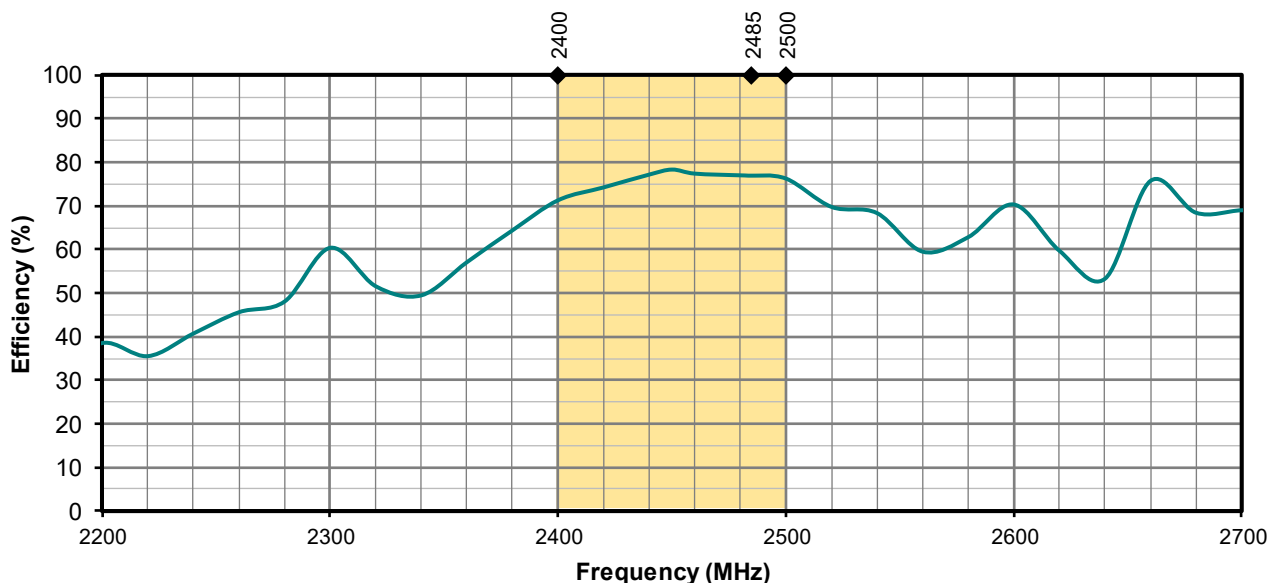
Figure 9. Antenna Efficiency, Straight, No ground plane
