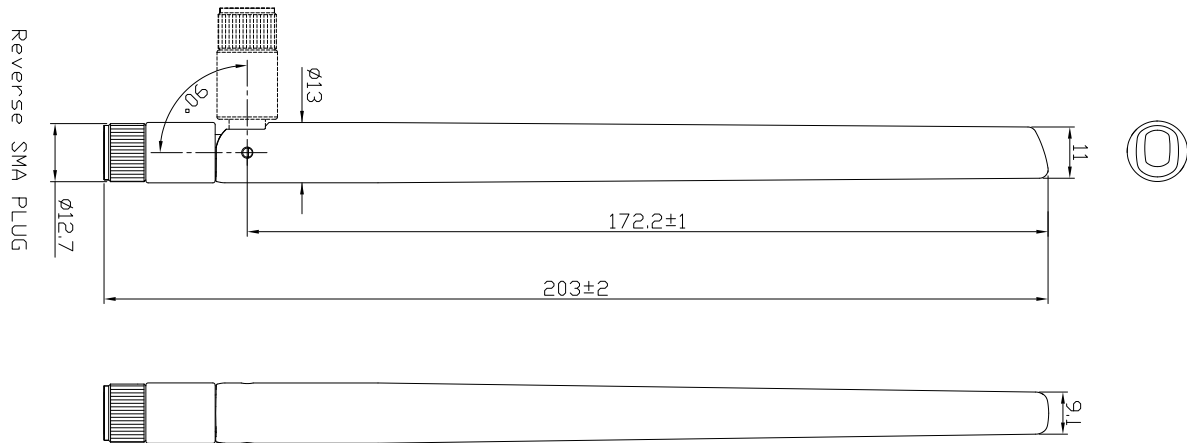
Figure 2. Antenna Dimensions
