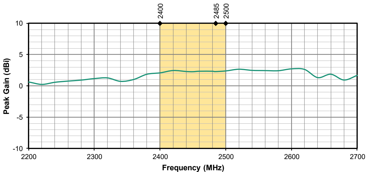
Figure 7. Antenna Peak Gain, Straight, No ground plane
