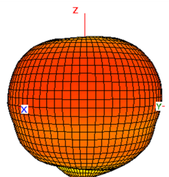
2500 MHz
