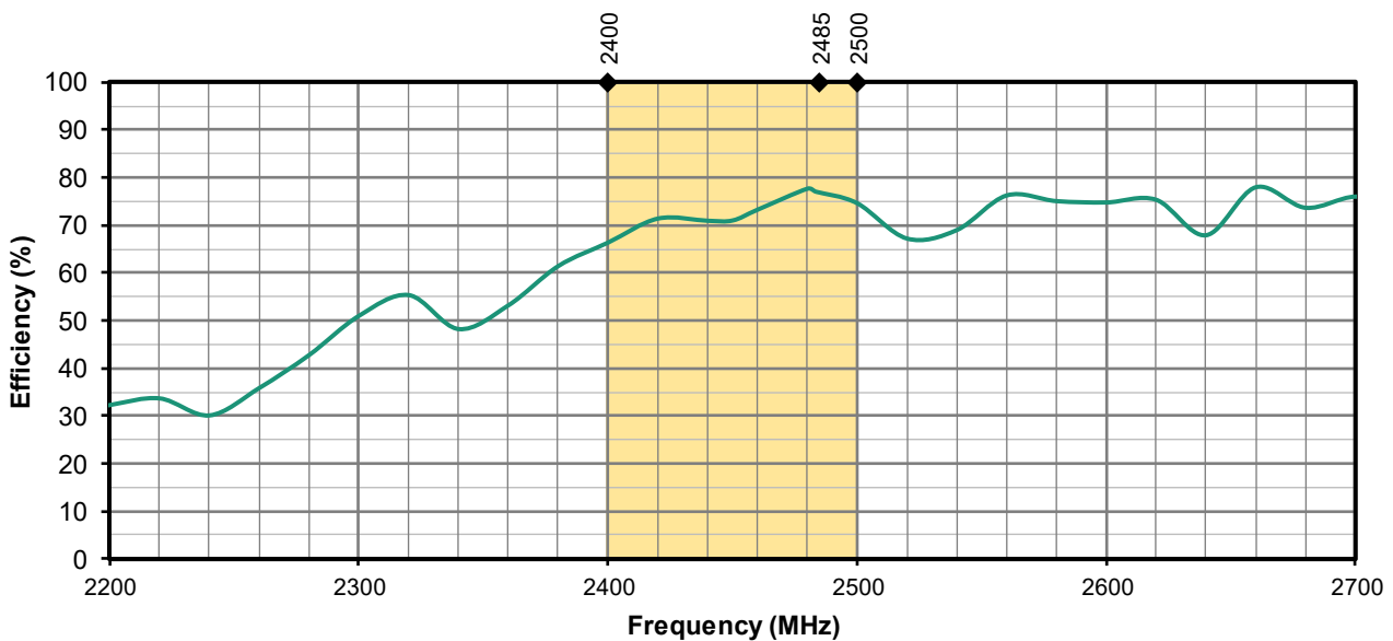
Figure 9. Antenna Efficiency, Straight, No ground plane
