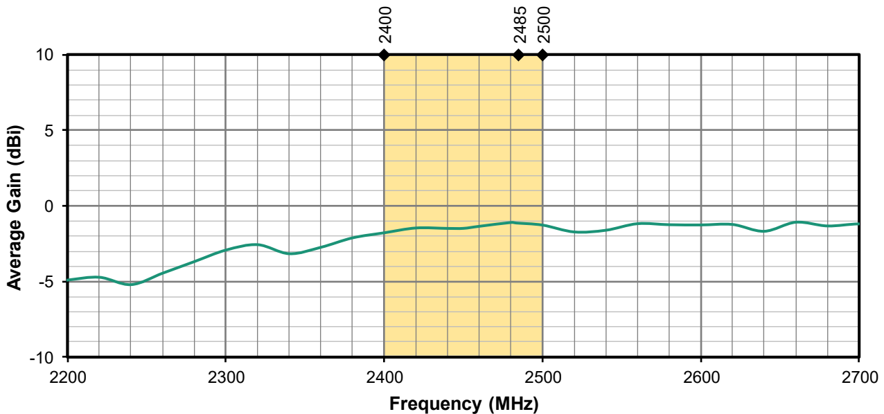
Figure 8. Antenna Average Gain, Straight, No ground plane
