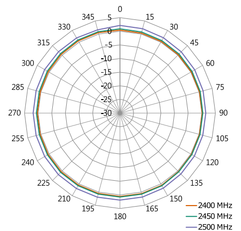
XY-Plane Gain
