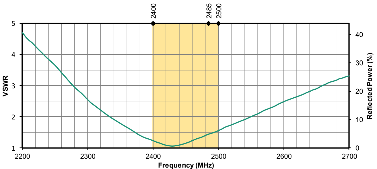
Figure 5. Antenna VSWR, Straight, No ground plane
