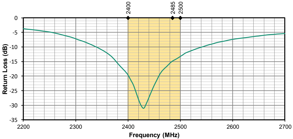
Figure 6. Antenna Return Loss, Straight, No ground plane
